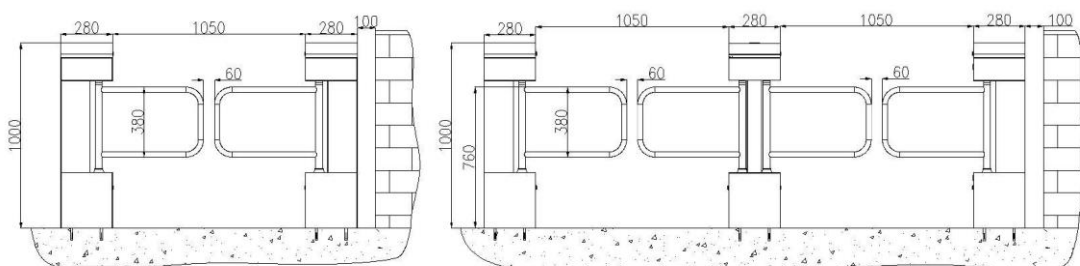
Figure2-2: STS2100B/2200B Single channel and dual channel
