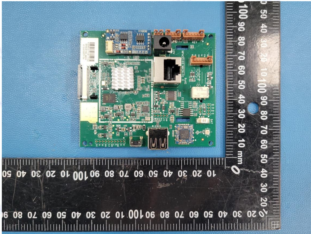
Photo 9: PCB view
