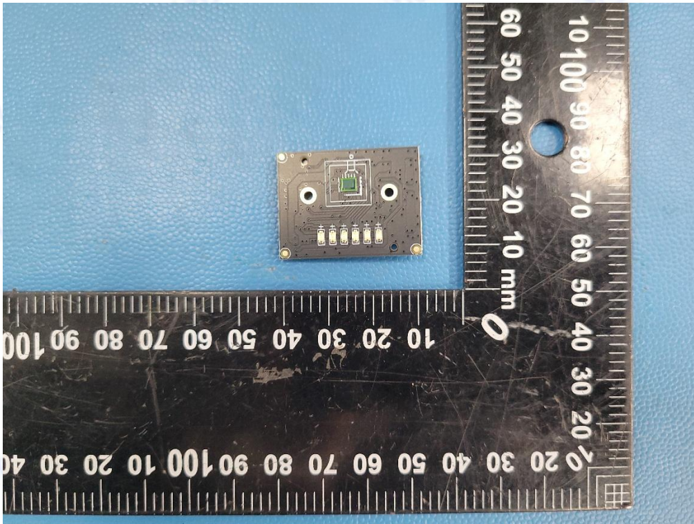
Photo 5: PCB view
