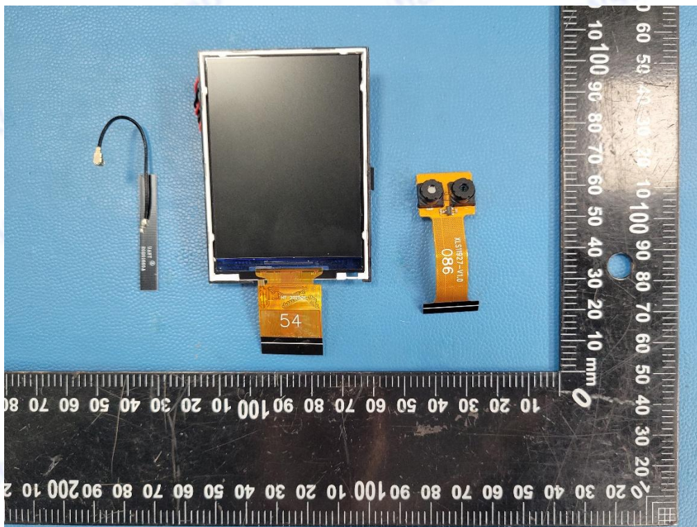
Photo 11: Component view
