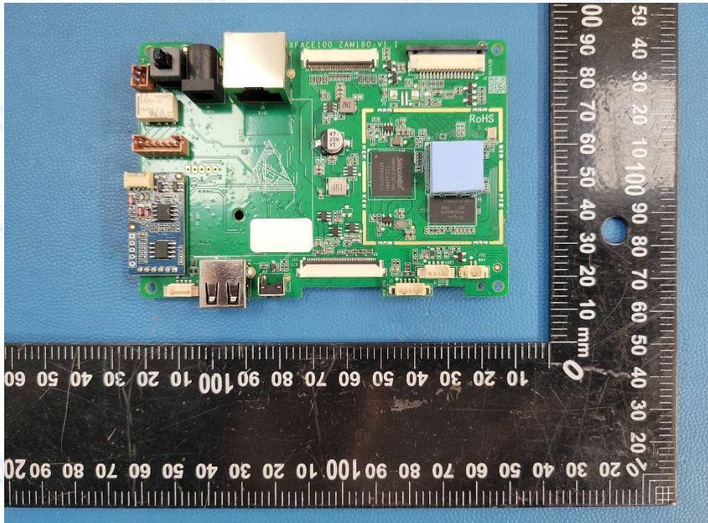
Photo 5: PCB view
