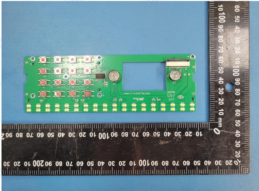
Photo 7: PCB view
