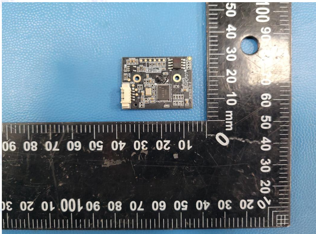
Photo 12: PCB view
