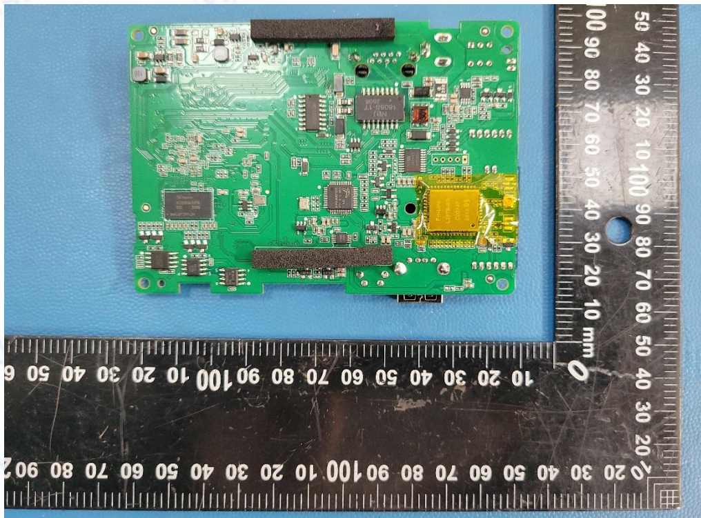
Photo 6: PCB view
