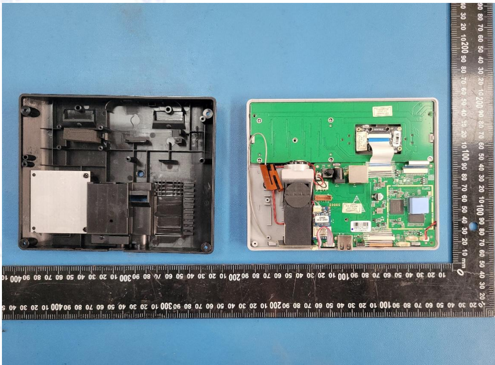
Photo 4: Internal view
