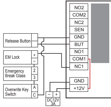
▶ Diagram 2 • Normally Open (NO)
