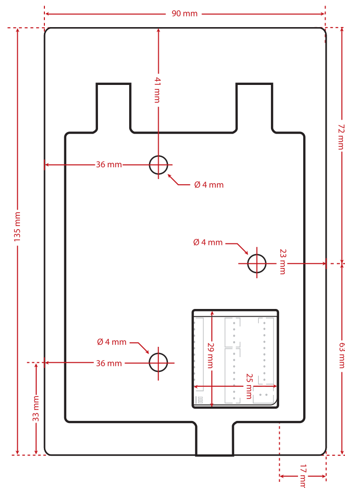
Front View of m-Kadex
