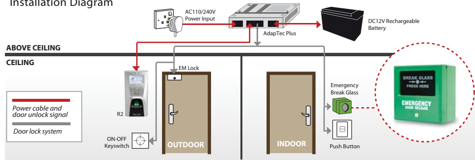
Installation Diagram
